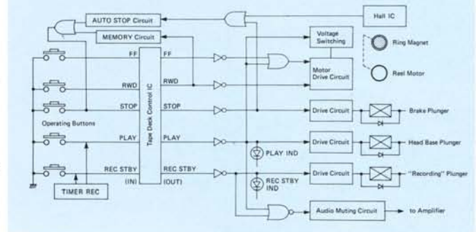
Logic-Control-Block-Diagramm
